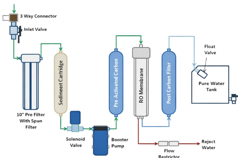
Process Flow Diagram
